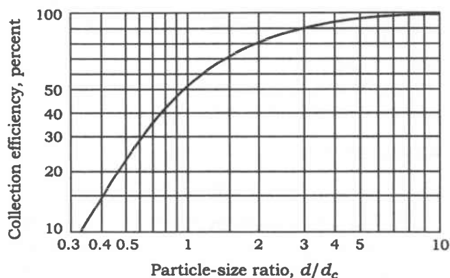
Cyclone efficiency
