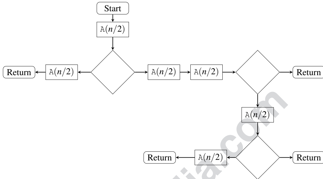
Flowchart for Recursive Function A(n)
